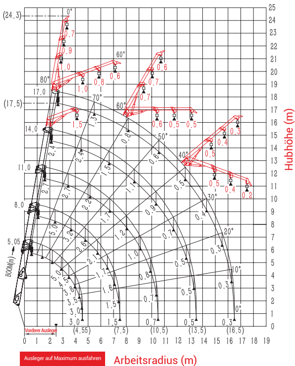
Lastdiagramm (t)
